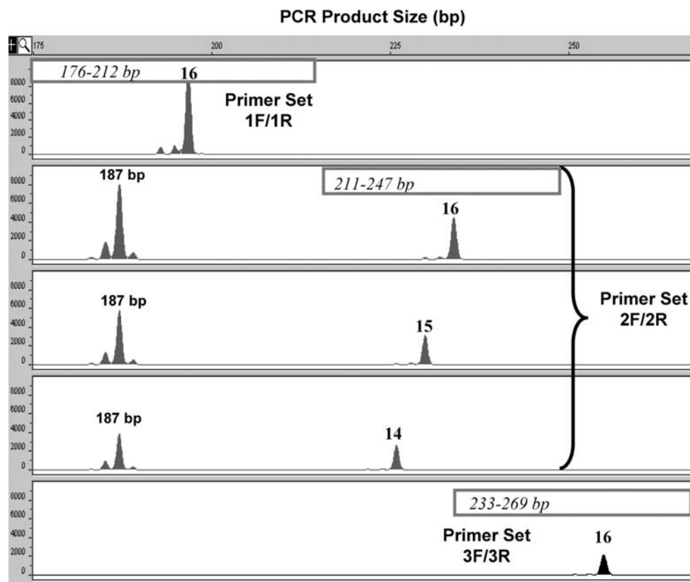
Fig. 1 Electropherograms of samples amplified with primer sets 1F/1R, 2F/2R, 3F/3R listed in Table 1. Amplification of male templates using sets 1F/1R and 3F/3R resulted only in the amplification of the DYS19 locus while primer set 2F/2R produced, in addition to the DYS19-specific product, an invariant amplicon at 187 bp that was specific to the AC006335 region. Numbers above the peaks indicate the DYS19 allele call
