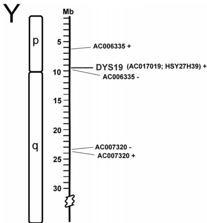
Fig. 2 Illustration of Y-chromosome positions for DYS19 locus and homologous regions discovered during a human BLAT search against the human genome reference sequence. The AC numbers describe sequence contigs present in GenBank with either forward (+) or reverse (–) orientations
