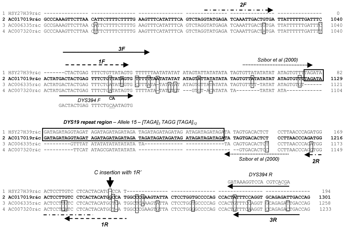
Fig.3 Sequence alignments for the DYS19 locus (HSY27H39 and AC017019) and its Y homologs (AC006335 and AC007320). Positions of primers used in this study (see Table 1) or other published ones are illustrated as horizontal arrows . The sequences are displayed as reverse and complement (r&c) so that “forward” and “reverse” primers and the repeat structure are in a familiar format. The homologs are nearly identical to the flanking regions of DYS19 but are missing the TAGA repeat region ( indicated by dashes ). Sequence differences between the various alignments are boxed . The vertical arrow near the 5'-end of primer 1R indicates an insertion of a single G in the AC017019 version of DYS19 relative to the original HSY27H39 sequence
